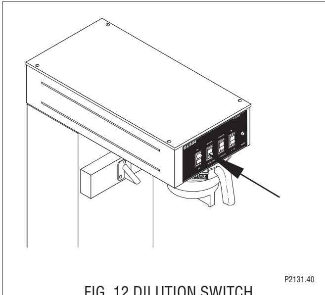
FIG. 12 DILUTION SWITCH
