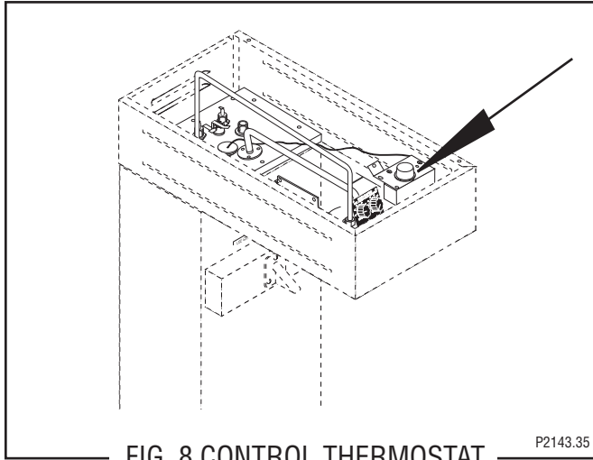
FIG. 8 CONTROL THERMOSTAT
