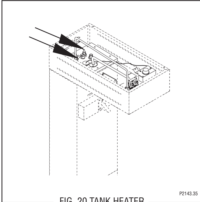
FIG. 20 TANK HEATER
