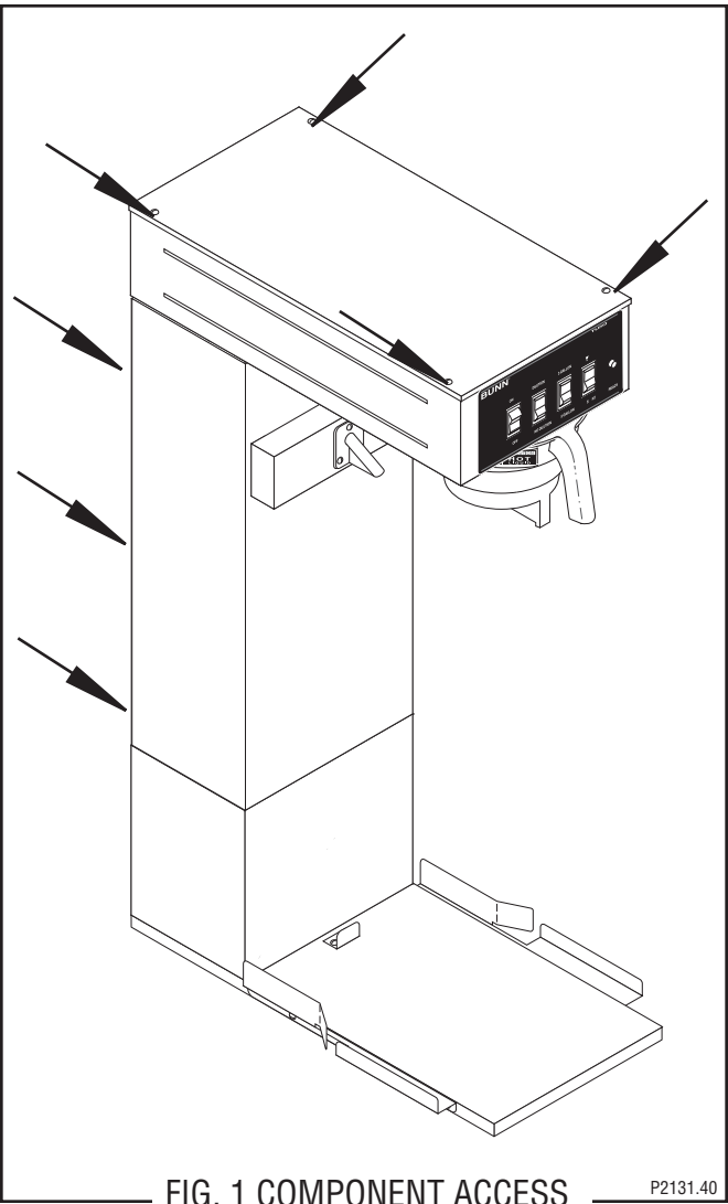
FIG. 1 COMPONENT ACCESS
