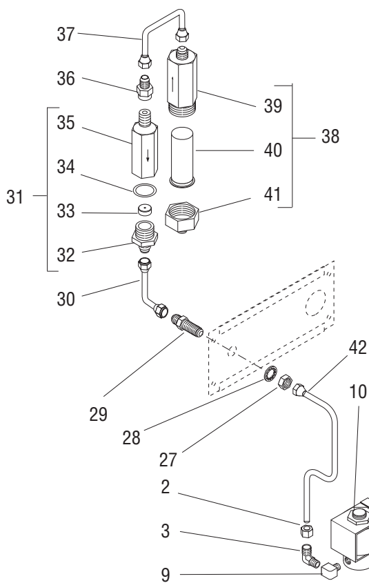
EARLY MODELS W/EXTERNAL MOUNTING
