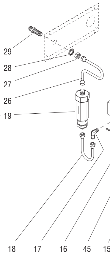
EARLY MODELS W/EXTERNAL MOUNTING
