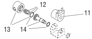
SOLENOIDS W/1" DIA COIL
