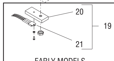
EARLY MODELS 20 AMP DISPENSERS
