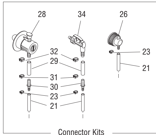
Connector Kits
