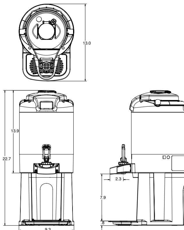
1.5 Gal TF Digital Server
