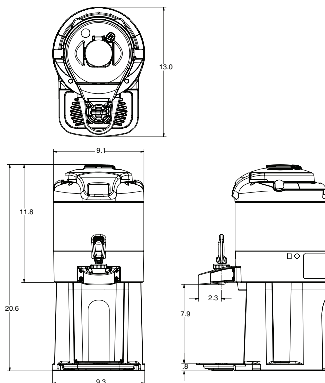
1 Gal TF Digital Server
