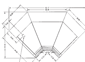
TOP VIEW SQROC90
