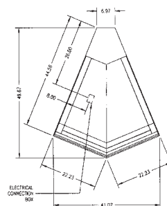
TOP VIEW SQROC45R
