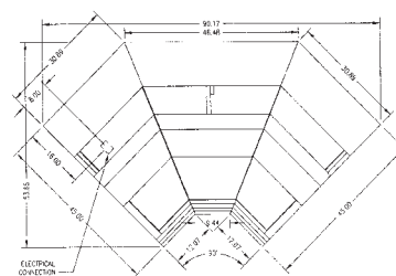
TOP VIEW SQRIC90
