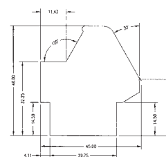
SIDE VIEW Service Case
