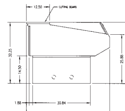
SIDE VIEW Self-Serve Case
