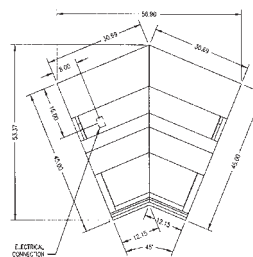
TOP VIEW SQRIC45R
