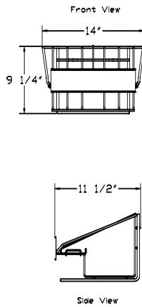
2 Pot Wide Rack (Part # 70577)
