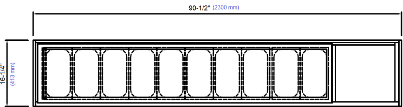
PLAN VIEW
