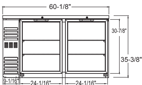
FRONT NLBB60NG
