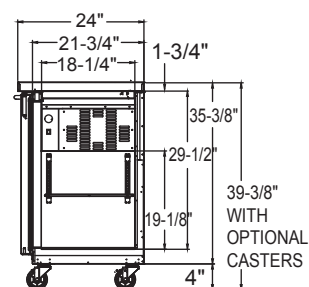
SIDE ALL MODELS
