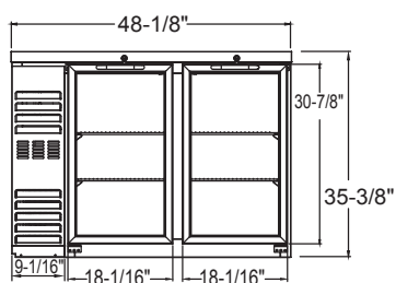
FRONT NLBB48NG
