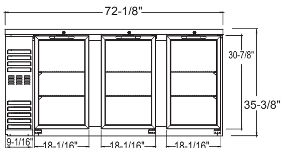
FRONT NLBB72NG
